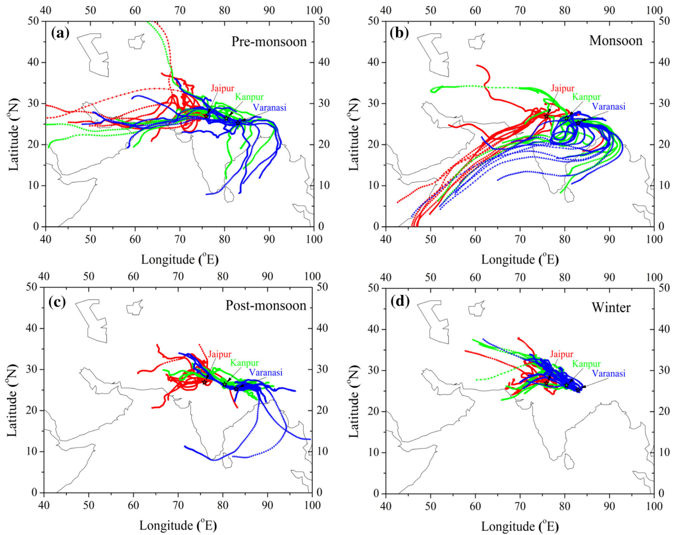
Fig. 6 Air mass back trajectories during a pre-monsoon, b monsoon, c post-monsoon, and d winter seasons at some higher aerosol loading days of year 2013
